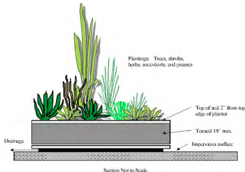
Figure 1: Stormwater Planter Section
