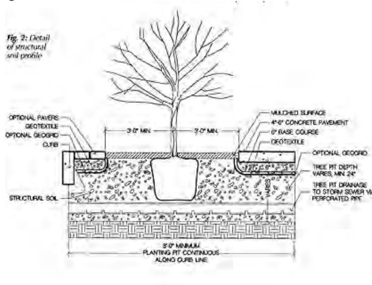
Figure 7: Section of a Tree Pit
