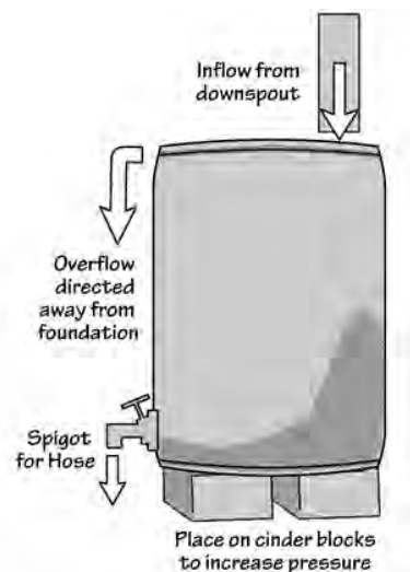
Figure 1: Rain Barrel Parts
