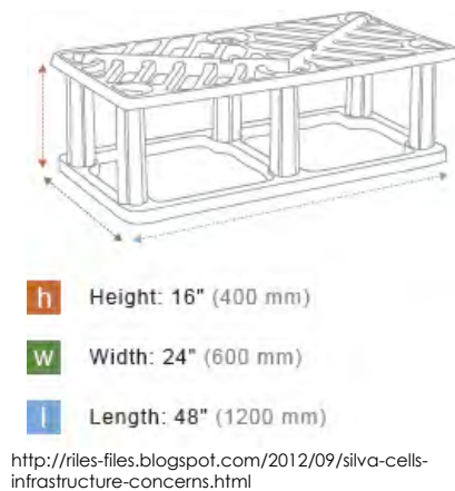
Figure 14: Silva Cell
